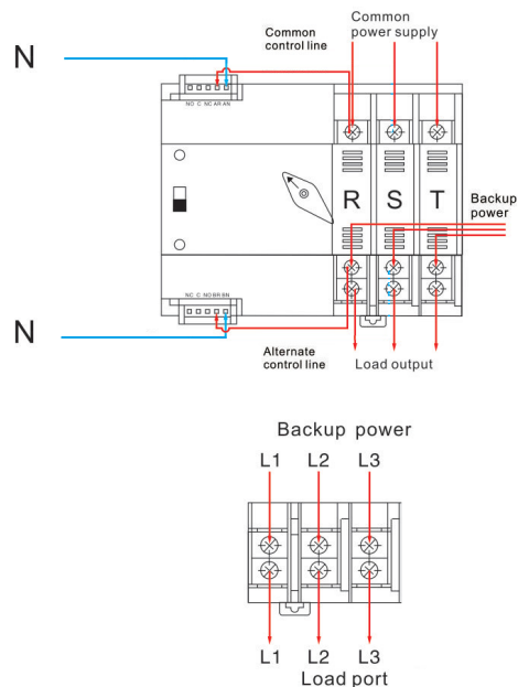
Fig.2 Wiring diagram of controller
